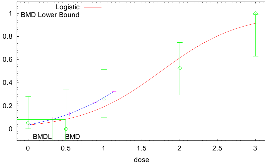
Logistic Model with 0.95 Confidence Level
